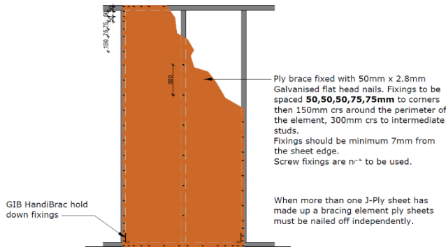
BP1 - CMPC Ply Structural Brace 1 side
