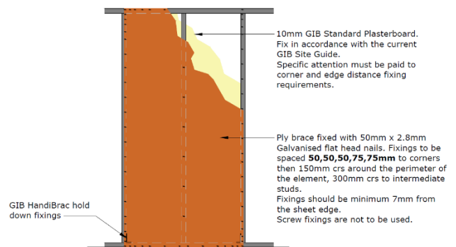
BPG - CMPC Ply Structural Brace 1 side with 10mm GIB Standard Plasterboard Lining other side
