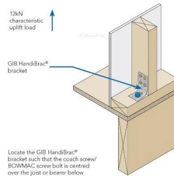
Timber Floor - External Wall
